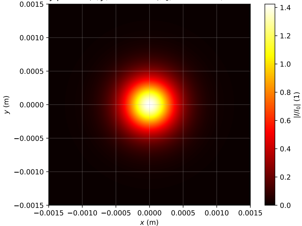
Intensity profile I(x, y, z = 3.901m)/I_0 , \text{Pin}=0.9\text{Pcr} , artificial time
